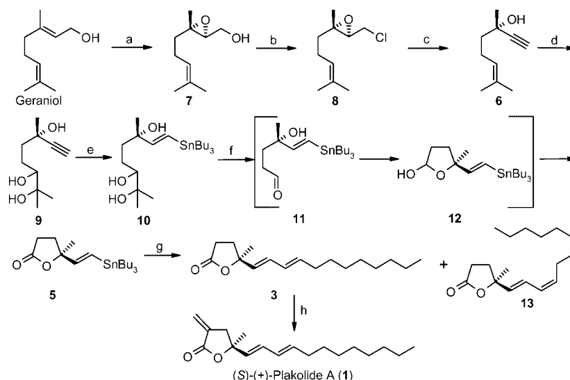
Scheme 1. Synthesis of (S)-(+)-Plakolide A ( 1 ). Reagents and conditions: (a) L-(+)-DIPT, \text{Ti}(\text{O}i\text{Pr})_4 , TBHP, MS 4 Å, \text{CH}_2\text{Cl}_2 , -23^\circ\text{C} , 6 h, 95%; (b) \text{PPh}_3 , \text{CCl}_4 , reflux, 6 h, 93%; (c) n -BuLi, THF, -40^\circ\text{C} , 1 h, 85%; (d) \text{OsO}_4 , NMO, acetone/water (1:4), room temp., 12 h, 92%; (e) \text{Bu}_3\text{SnH} , AIBN, toluene, 110^\circ\text{C} , 6 h, 90%; (f) (1) silica gel supported \text{NaIO}_4 , \text{CH}_2\text{Cl}_2 , 1 h; (2) PDC, \text{CH}_2\text{Cl}_2 , 4 h, 84% over two steps; (g) 4 , \text{Pd}(\text{PPh}_3)_4 , LiCl, CuCl, DMSO, room temp. to 60^\circ\text{C} , 26 h, 83% for 3 and 9% for 13 ; (h) (1) LDA, THF, -78^\circ\text{C} , 15 min, (2) Eschenmoser's salt, -78^\circ\text{C} to room temp., 6 h, (3) \text{CH}_3\text{I} , \text{CH}_3\text{OH} , room temp., 18 h, 82%.
