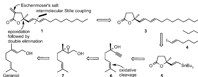
Figure 2. Retrosynthetic analysis of ( S )-(+)-Plakolide A (1).
